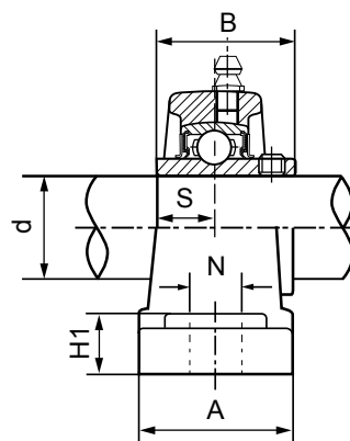
Standard B Type Seal
